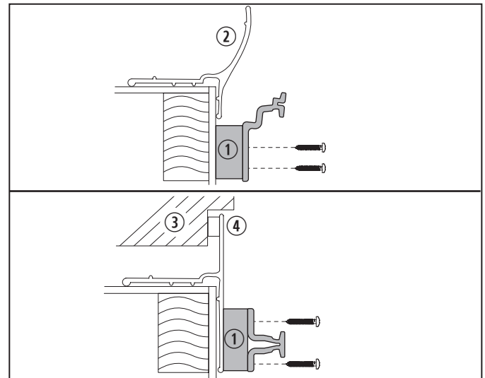
4 Optional Mounting Bracket Spacer
