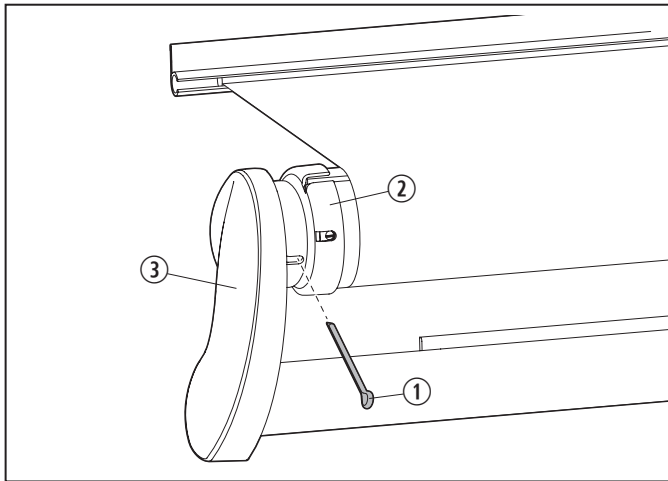
12 Removing the Cotter Pin
