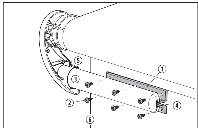
10 Securing the Mounting Bracket
