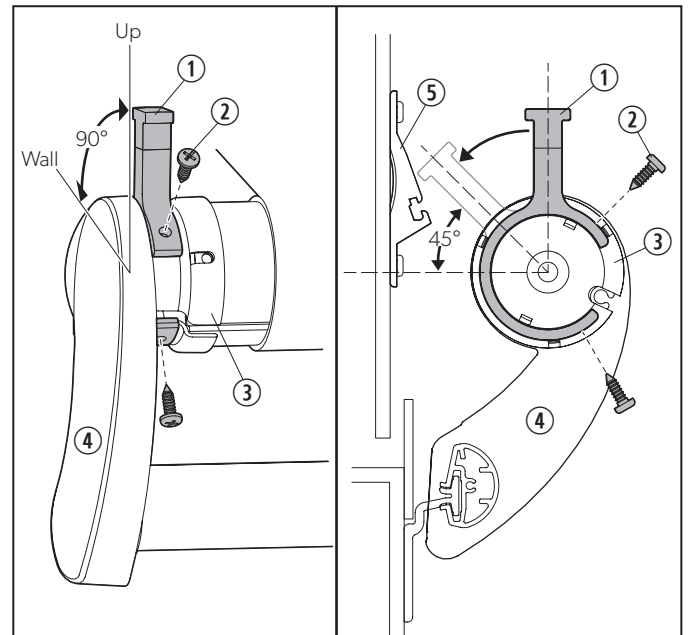
13 Installing and Positioning the Anti-Billow Stop
