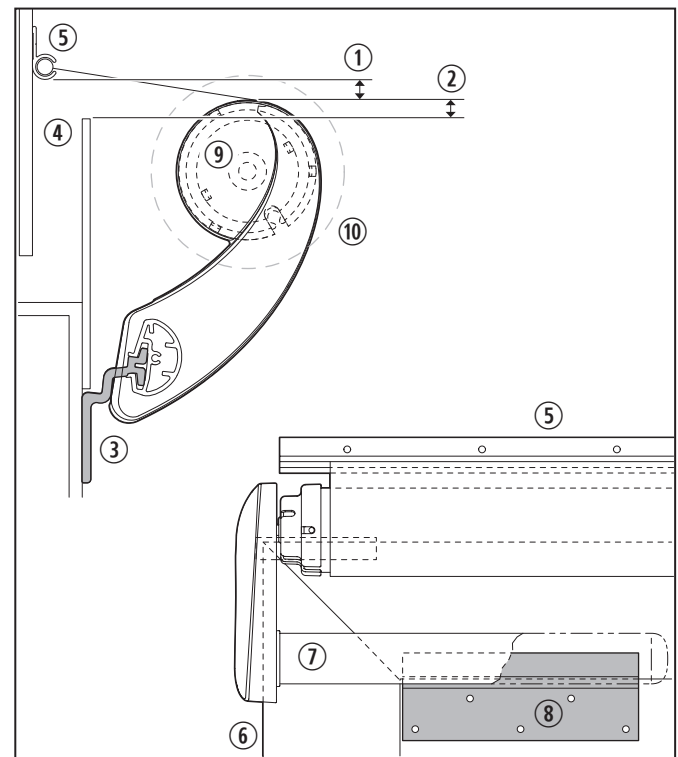
2 Tall Mounting Bracket Clearance
