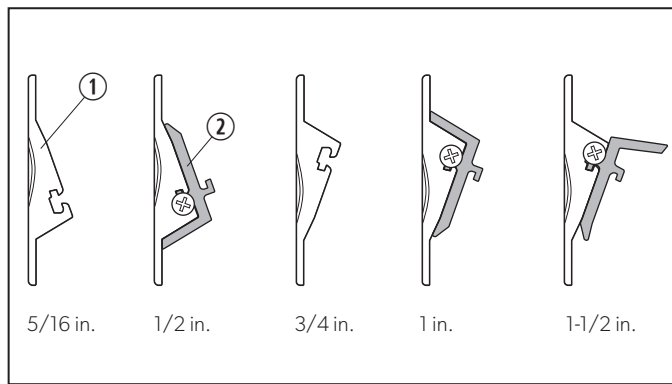
14 Configurations for the Anti-Billow Bracket and Spacer
