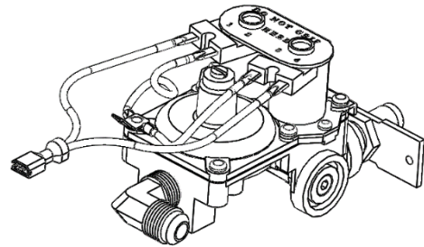
Figure 4 Valve Kit 31096
