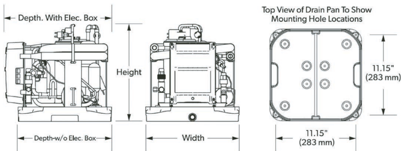
Dimensions DEGX6–16
