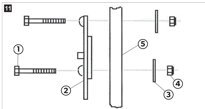
1 5/16 in bolt
