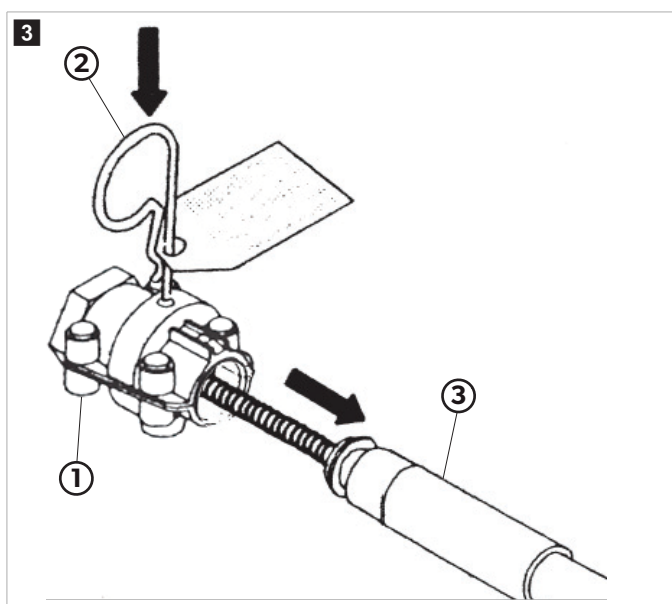
1 Helm 3 Cable body 2 Hitch pin
