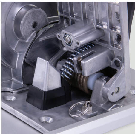
2. Stainless Steel Torsion Spring to Provide a Long Life
