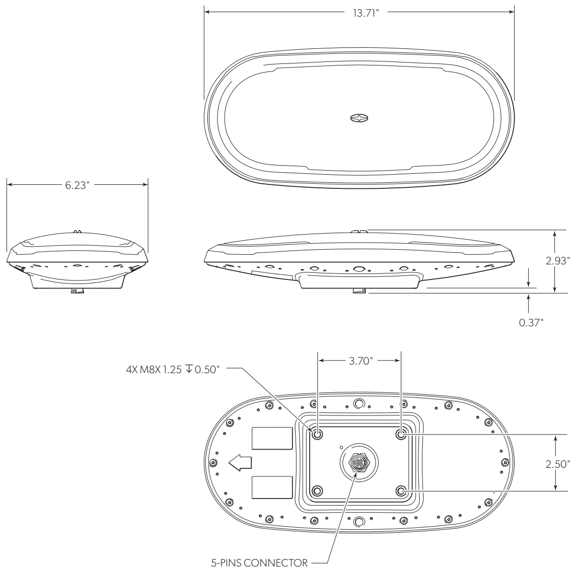
Figure 10-27. Sensor dimensions without mounting hardware.
