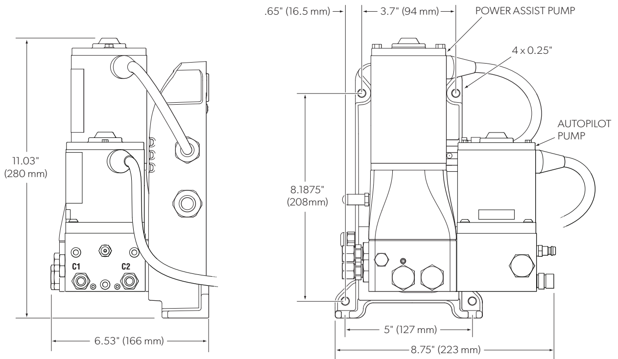
Figure 6-8. Dimensions shown with PA, AP, and retrofit kit part # HA1205.
