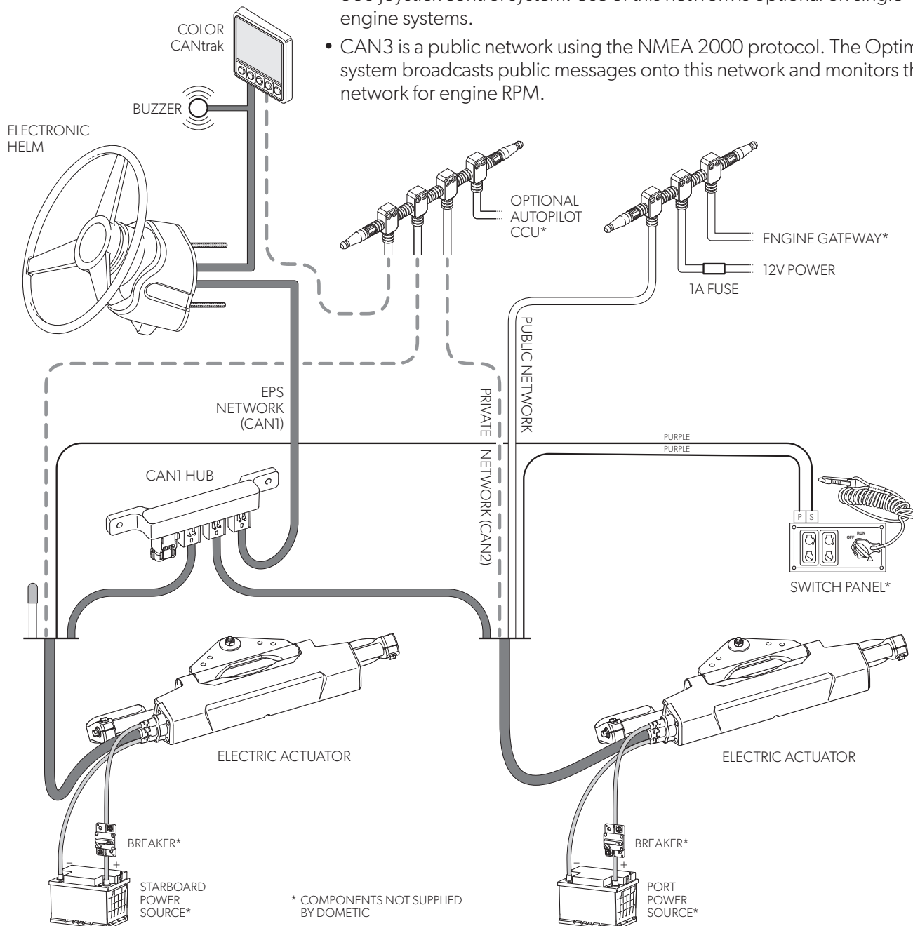
Figure 10-2. Optimus EPS electric actuator system diagram, single station, twin engine.
