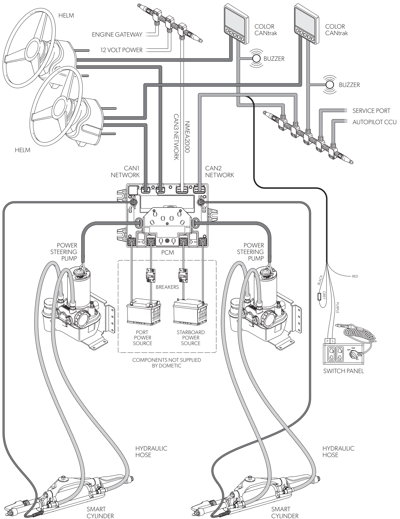
Figure 10-17. Optimus EPS electro/hydraulic system diagram, dual station, twin engine.
