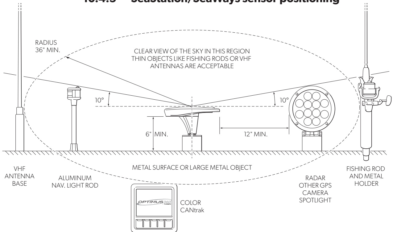
Figure 10-26. Sensor mounting distance from nearby VHF antennas and other equipment.
