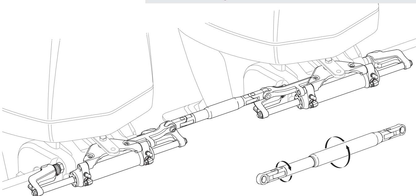
Figure 3-17. Twin engine, dual cylinder tie bar kit part # HA5520.
