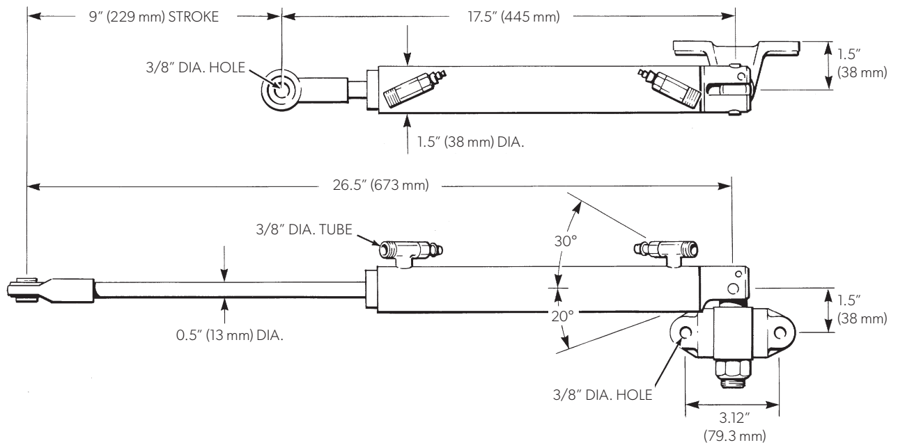
Figure 3-36. Splashwell mount cylinder part # HC5380-3.
