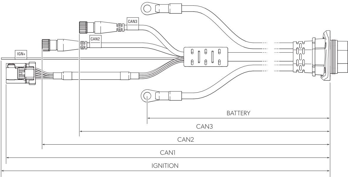
Figure 10-7. Nominal harness lengths.
