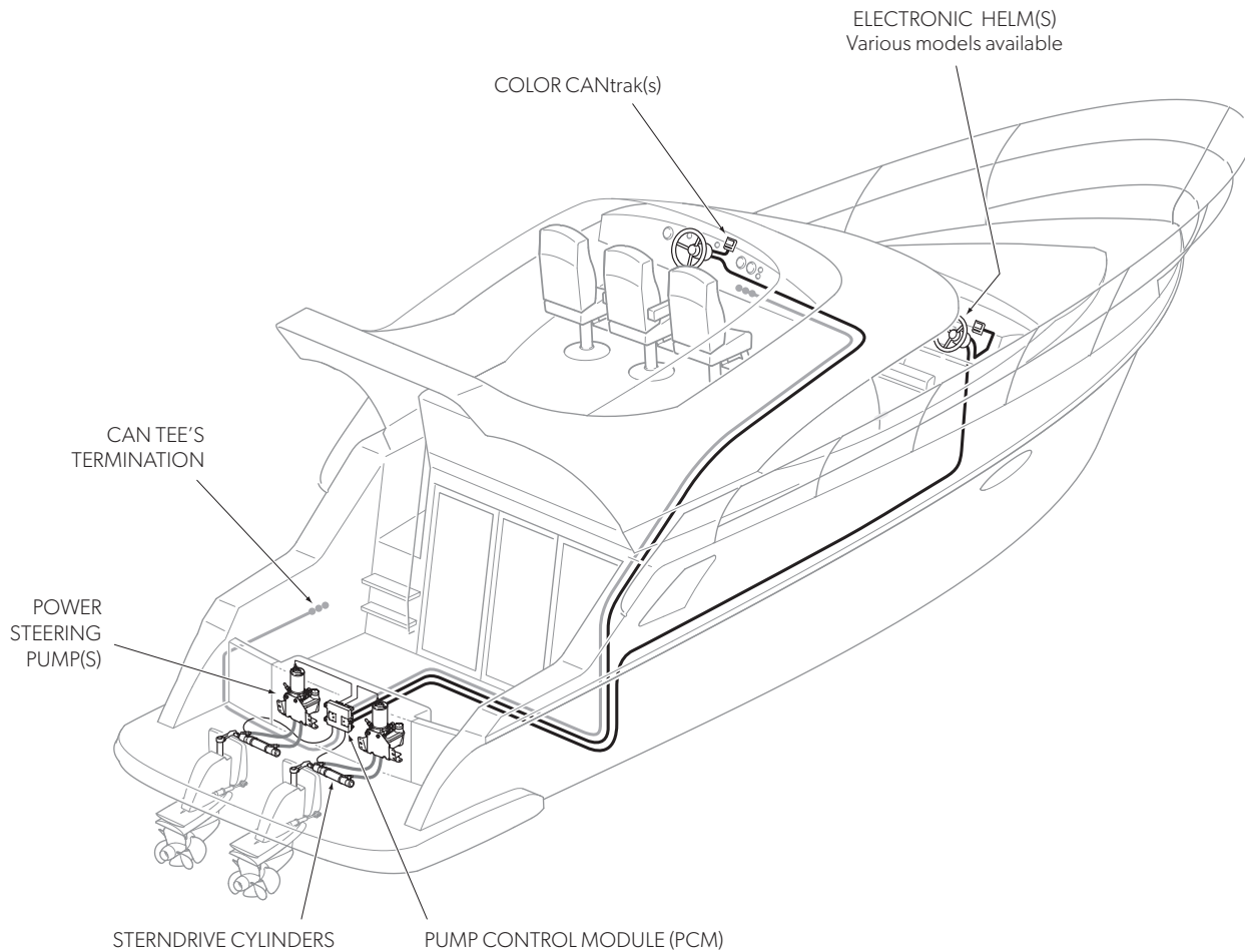
Figure 11-14. System components.
