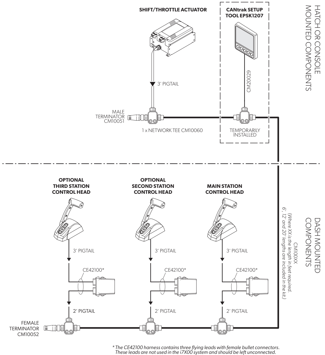
Figure 14-13. CAN2 wiring diagram, triple station, single engine.
