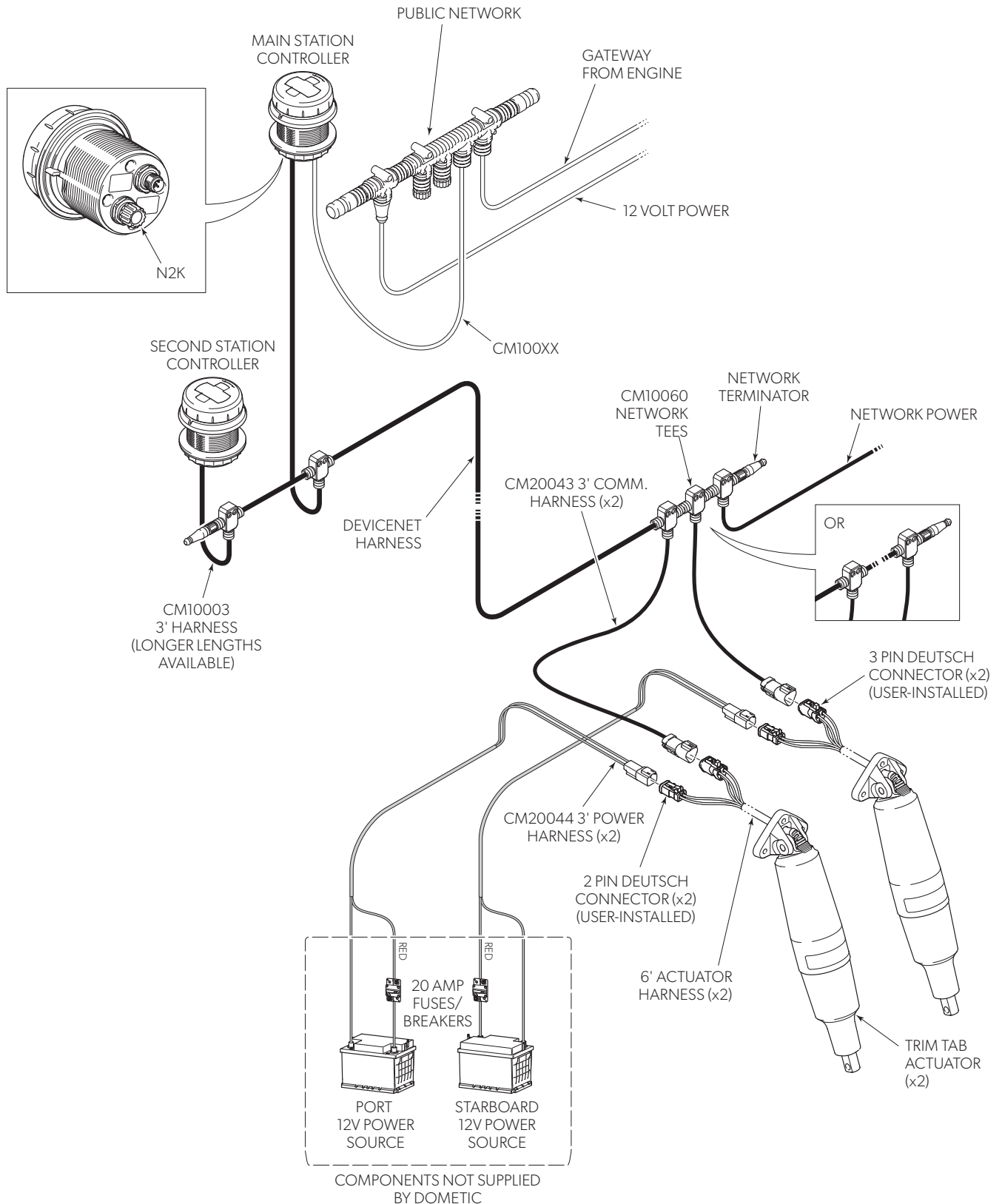
Figure 12-11. Dual station (adaptive series shown).
