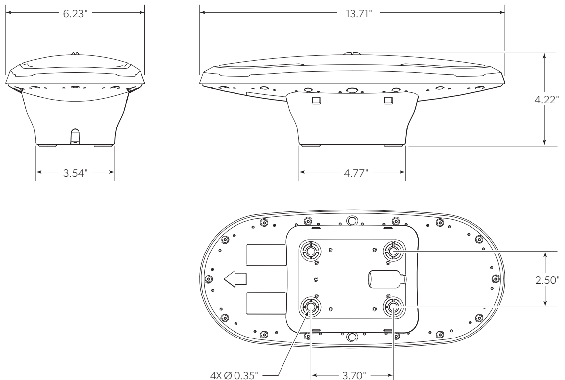
Figure 10-29. Sensor with high profile mount accessory dimensions.
