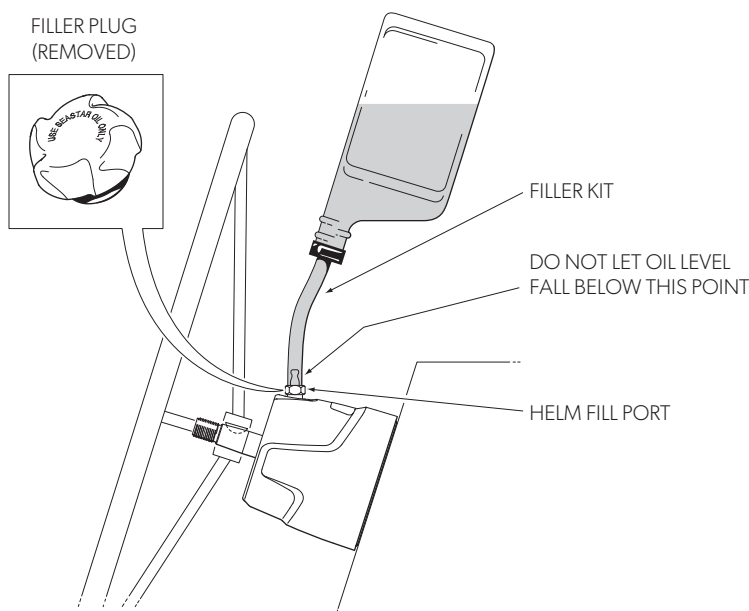
Figure 8-3. Fluid fill kit part# HA5438.
