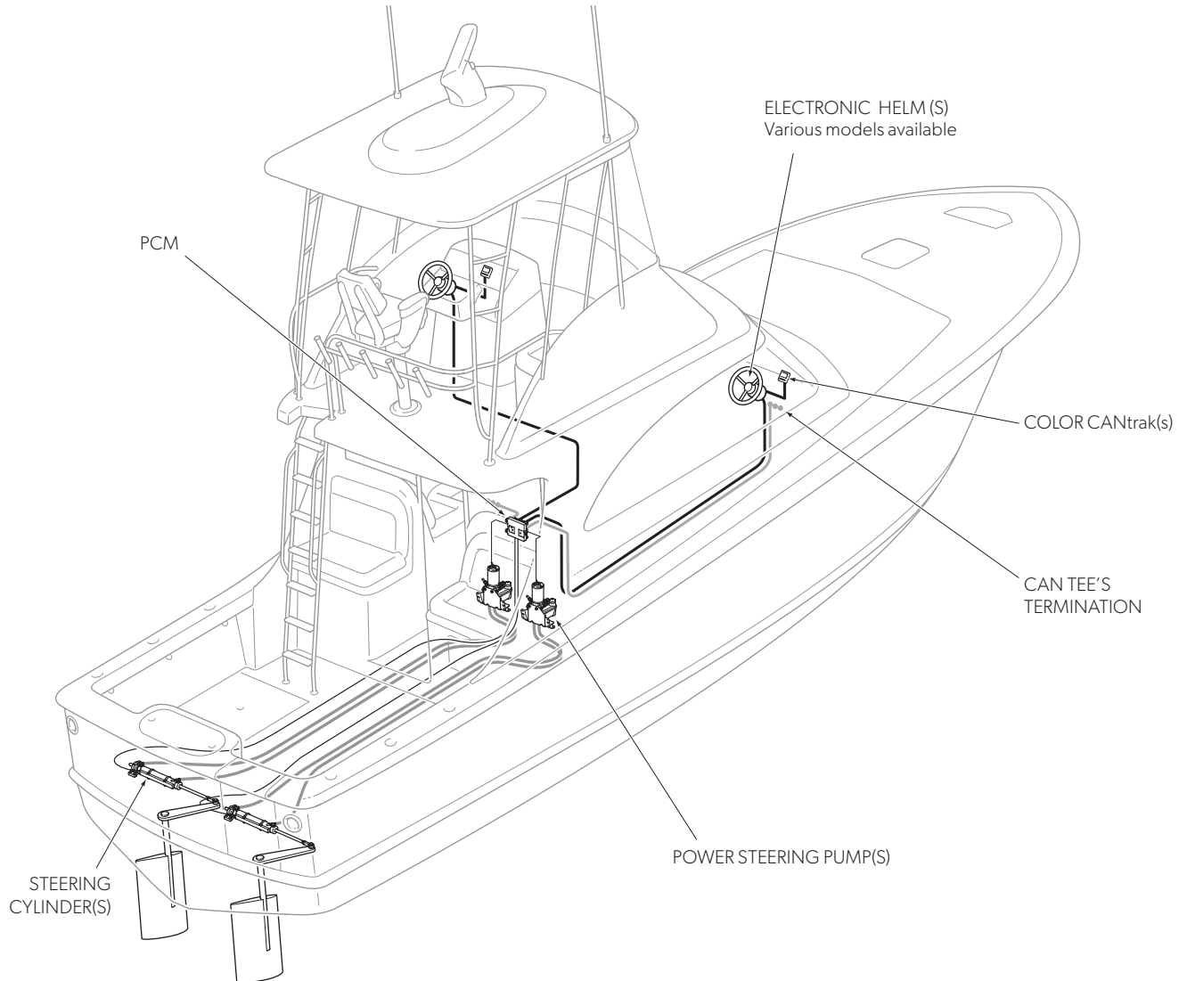
Figure 11-5. System components. Twin rudder system shown. * Subject to submission of survey form and rudder load calculation.
