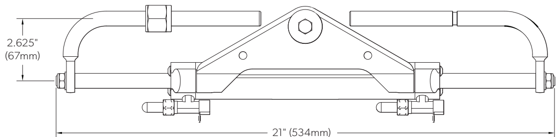
Figure 3-6. BayStar cylinder part # HC4645-3 / 47-3 / 58-3.
