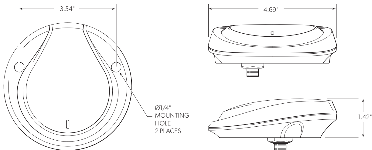
Figure 10-31. SeaWays GO sensor dimensions.
