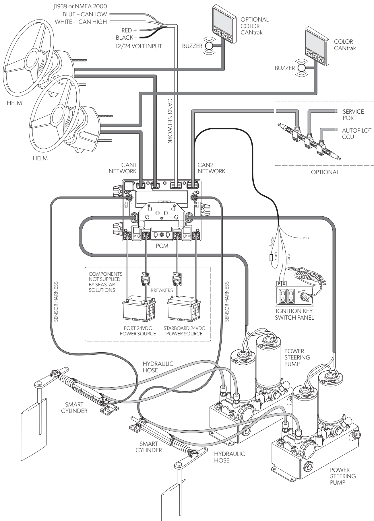
Figure 11-10 . Optimus EPS system diagram, dual station, dual cylinder (twin rudders).
