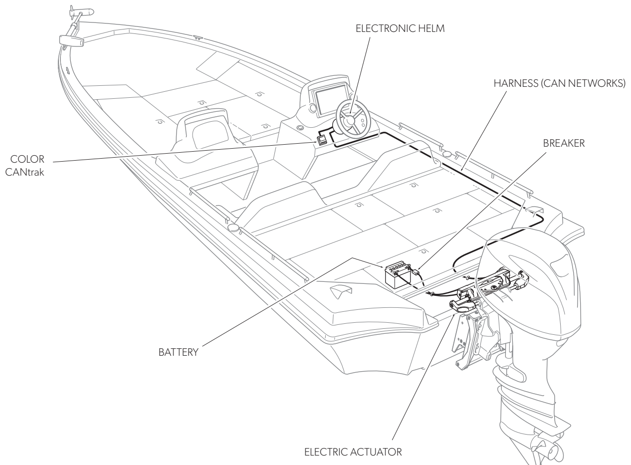
Figure 10-8. Electric bass boat (for reference only).
