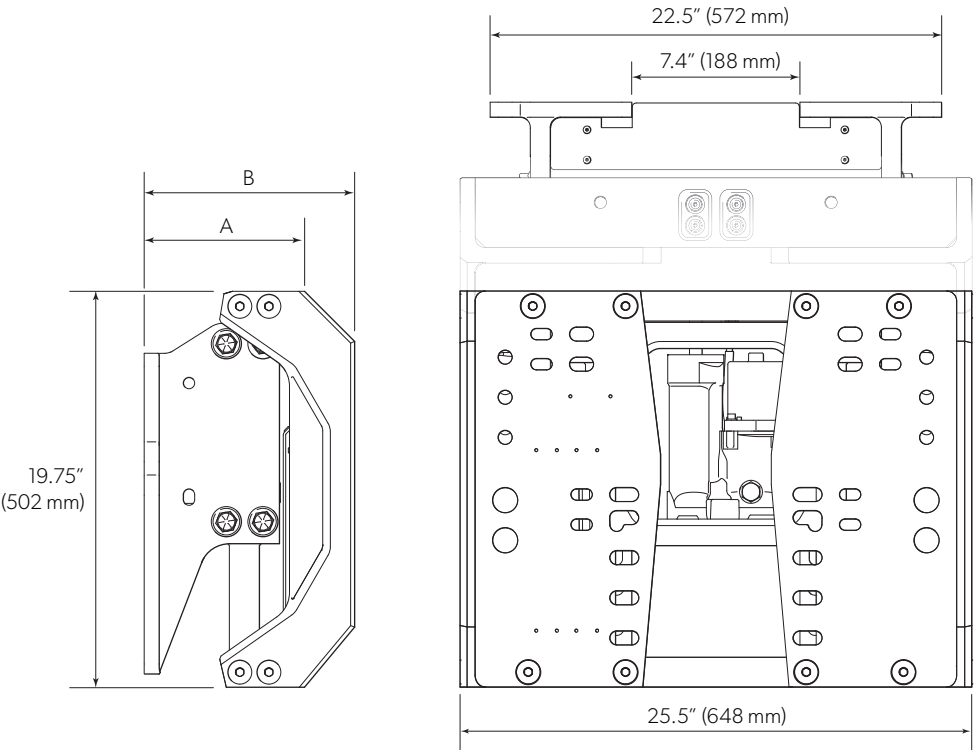
Figure 13-6. Wide (Mercury) Mega jack plate — also accepts Standard mounting engines.
