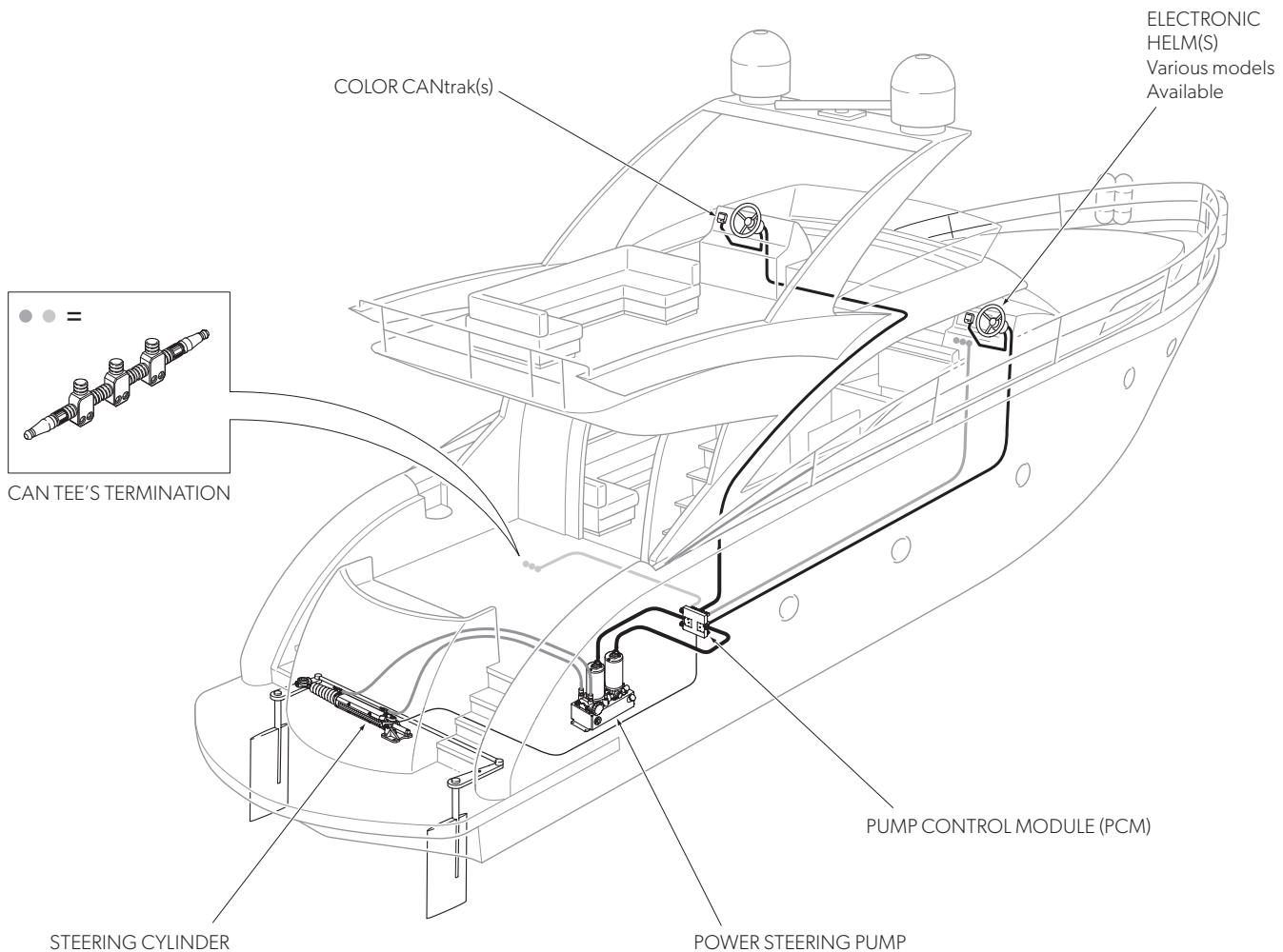
Figure 11-8. System components, dual station, single cylinder (twin rudders).
