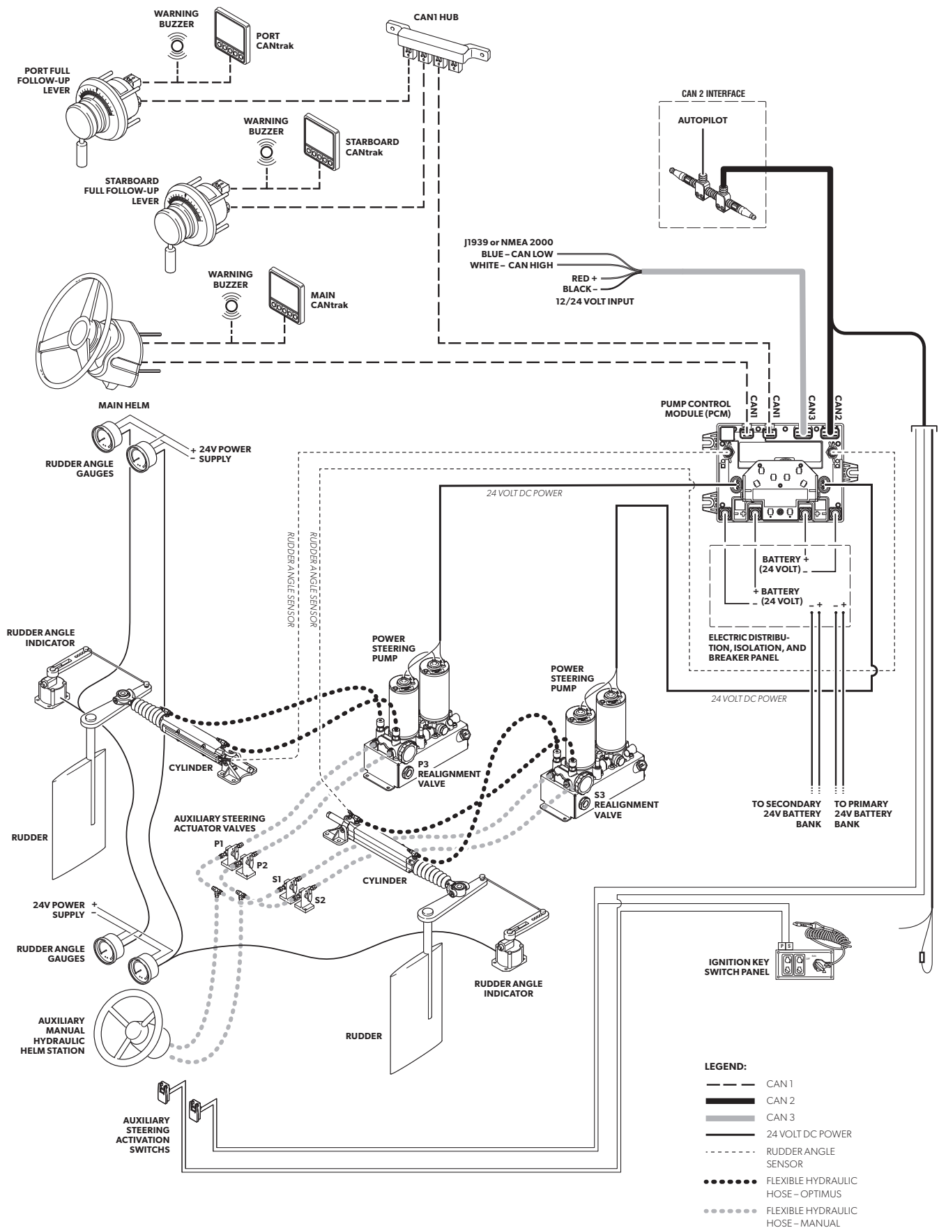
Figure 11-13 . Optimus EPS system diagram, class system with port and starboard wing stations.
