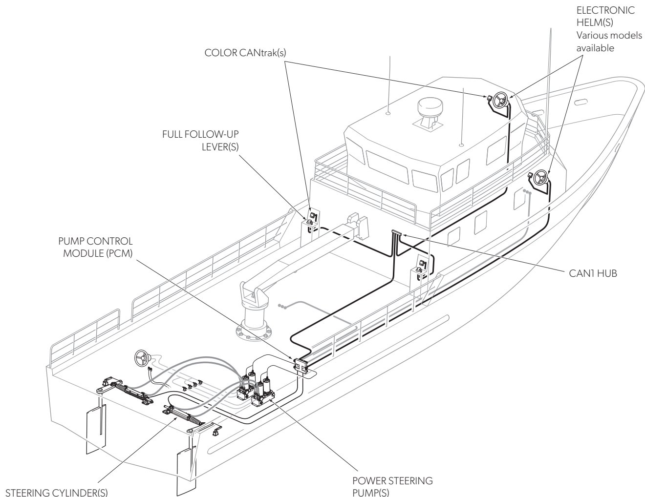
Figure 11-11. System components.
