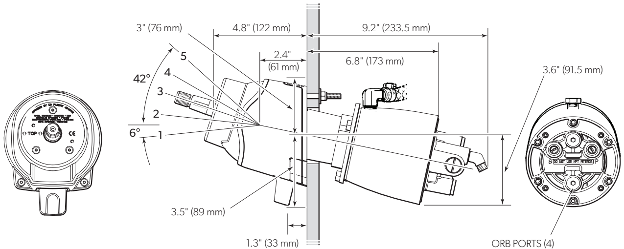
Figure 3-4. Sport tilt helm part # HH4315-4.
