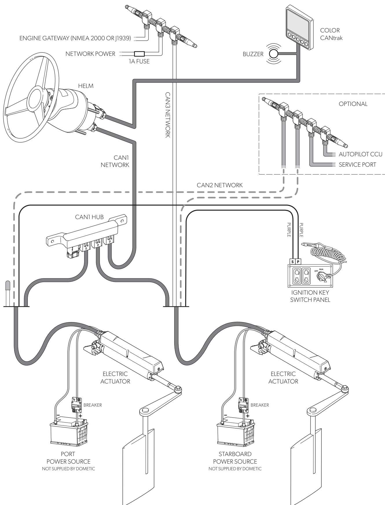
Figure 10-13. Electric inboard system diagram, dual actuator (for reference only).
