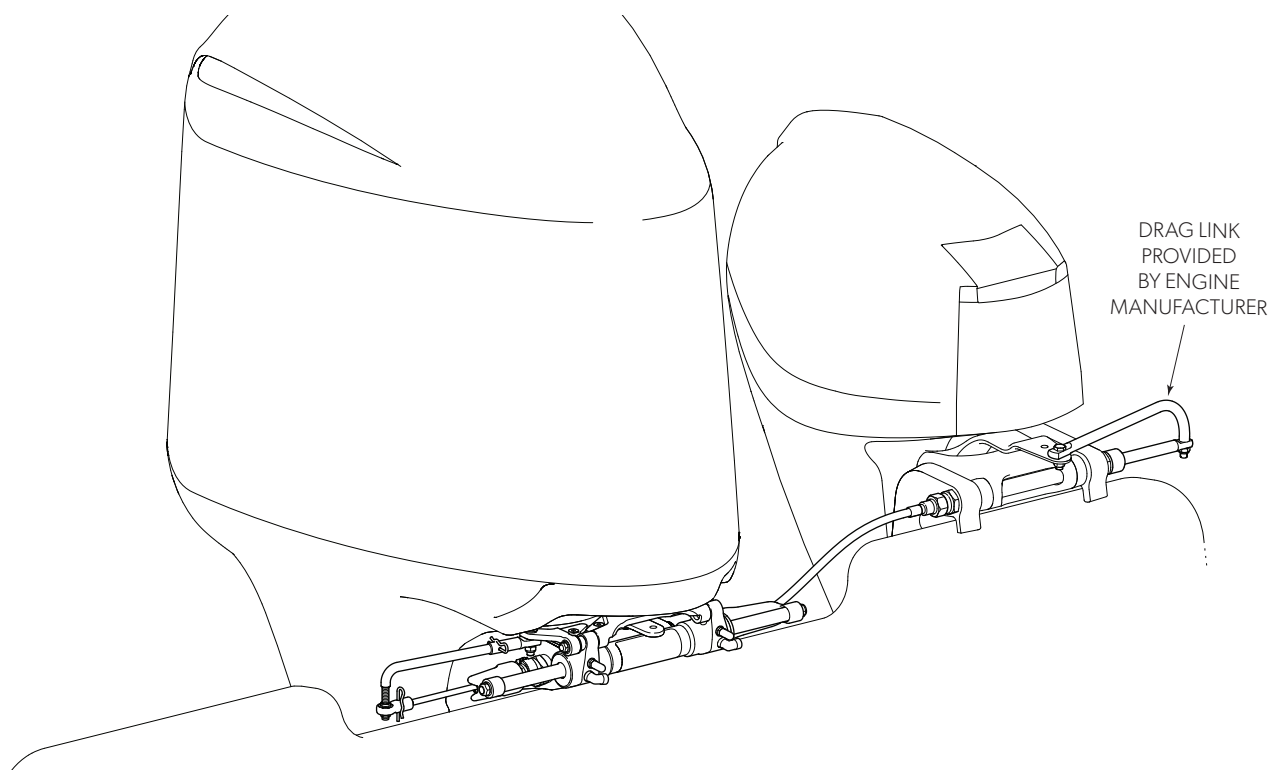
Figure 3-37. Kicker cable tie bar.
