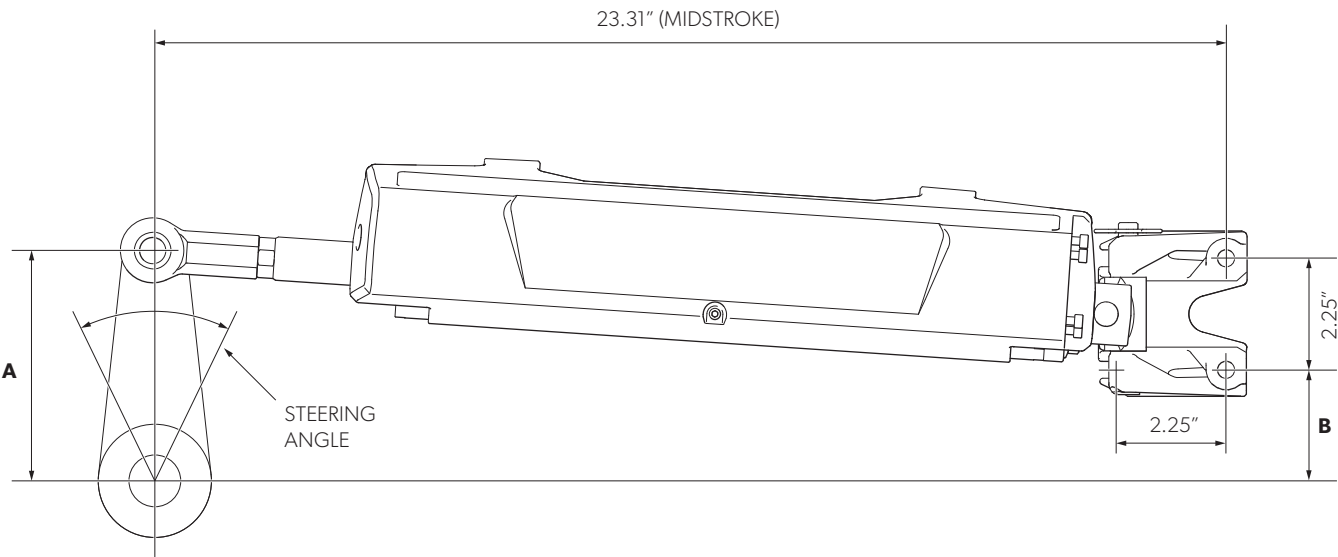
Figure 10-10. Electric inboard actuator EA3000 dimensions.
