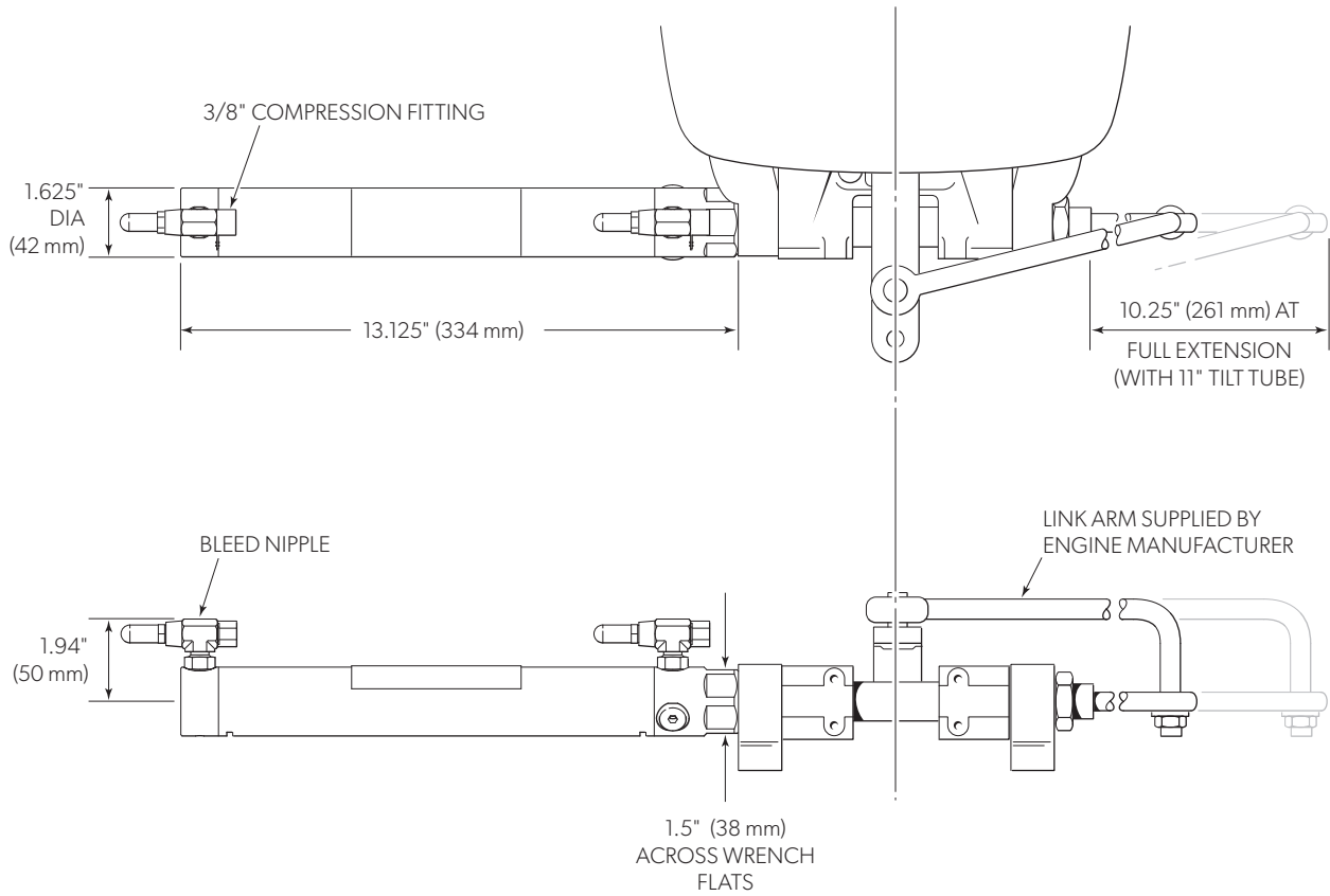
Figure 3-33. Side mount cylinder part # HC5370-3.
