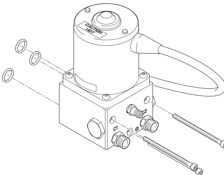
Figure 6-6. Retrofit kit part # HA1205.
