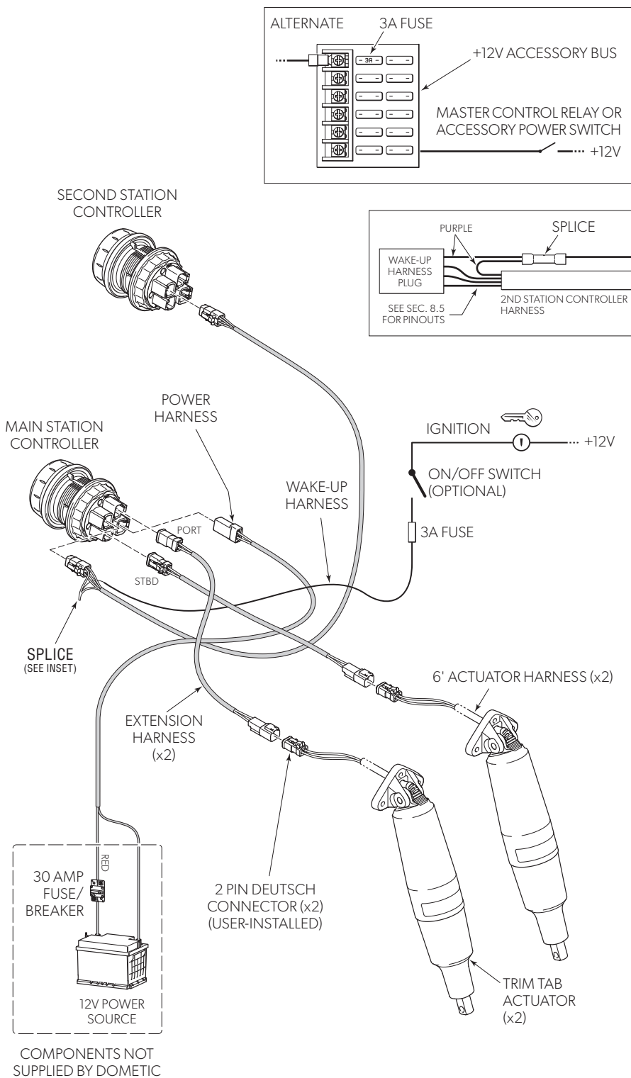
Figure 12-8. Dual station (standard series shown).
