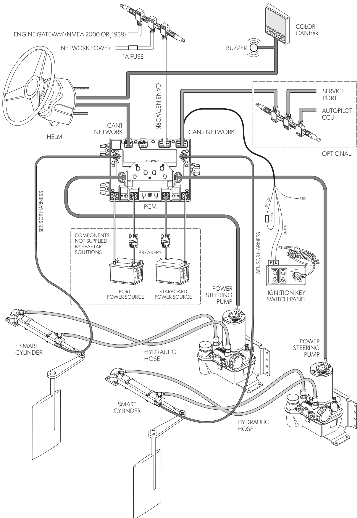
Figure 11-4. Optimus EPS system diagram, single station, twin rudder.
