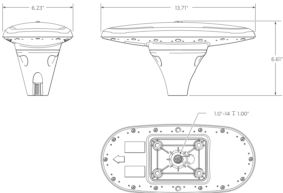
Figure 10-30. Sensor with pole mount accessory dimensions.
