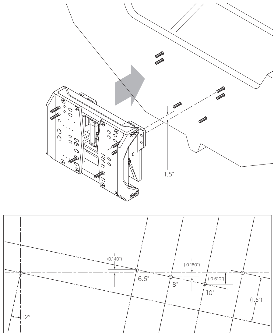
Figure 13-8. Engine lift per setback — Wide (Mercury) Mega jack plate. Not to scale.
