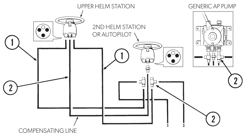
Figure 9-7. Note: Tee can be in helm or AP pump.
