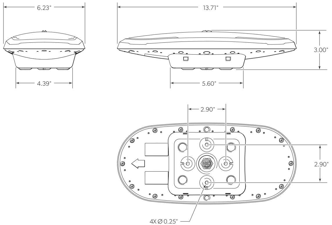
Figure 10-28. Sensor with low profile mount accessory dimensions.
