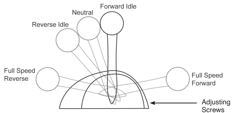
Figure 14-9. Control head lever positions.
