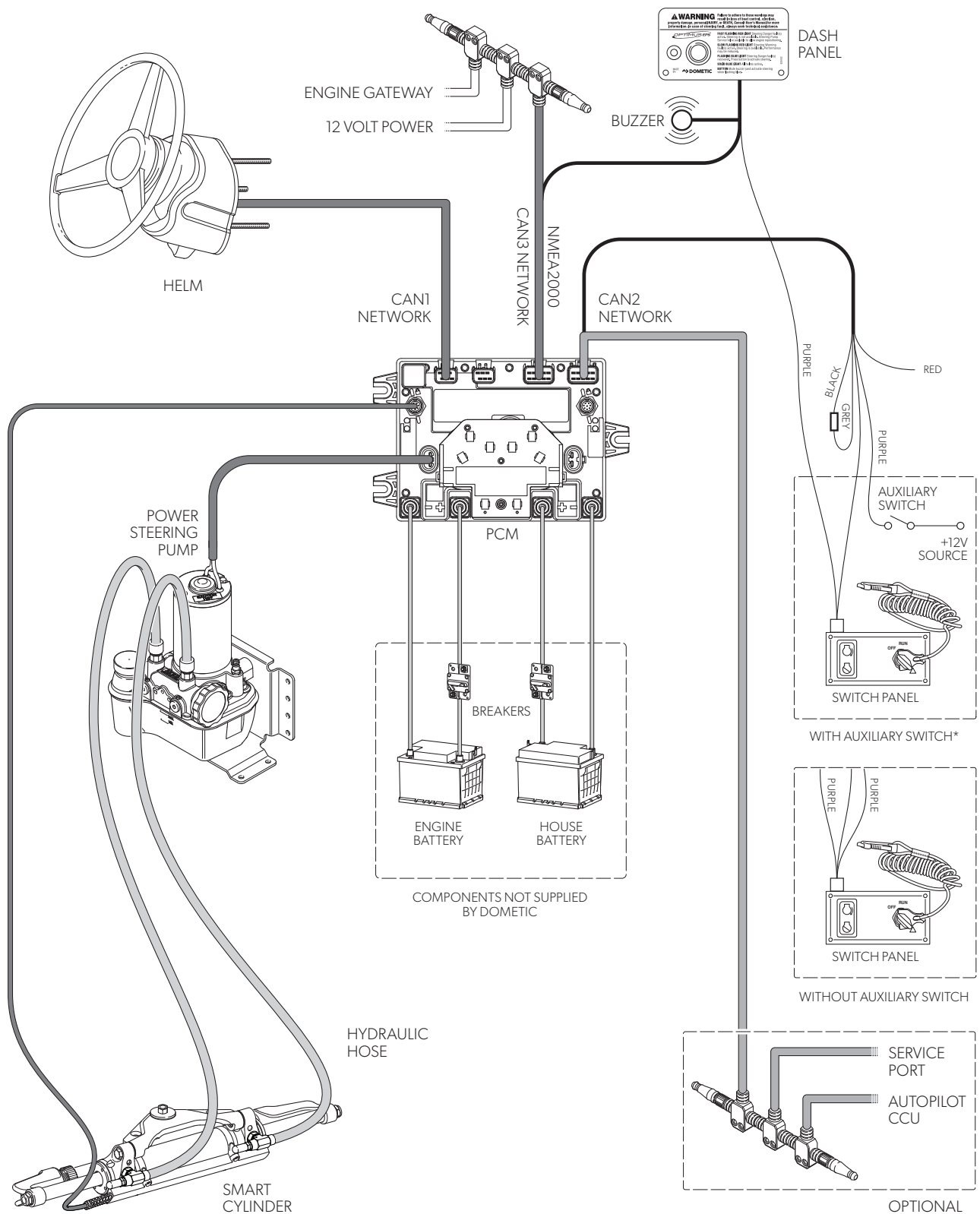
Figure 10-14. Optimus EPS electro/hydraulic system diagram, single station, single engine, with dash panel.
