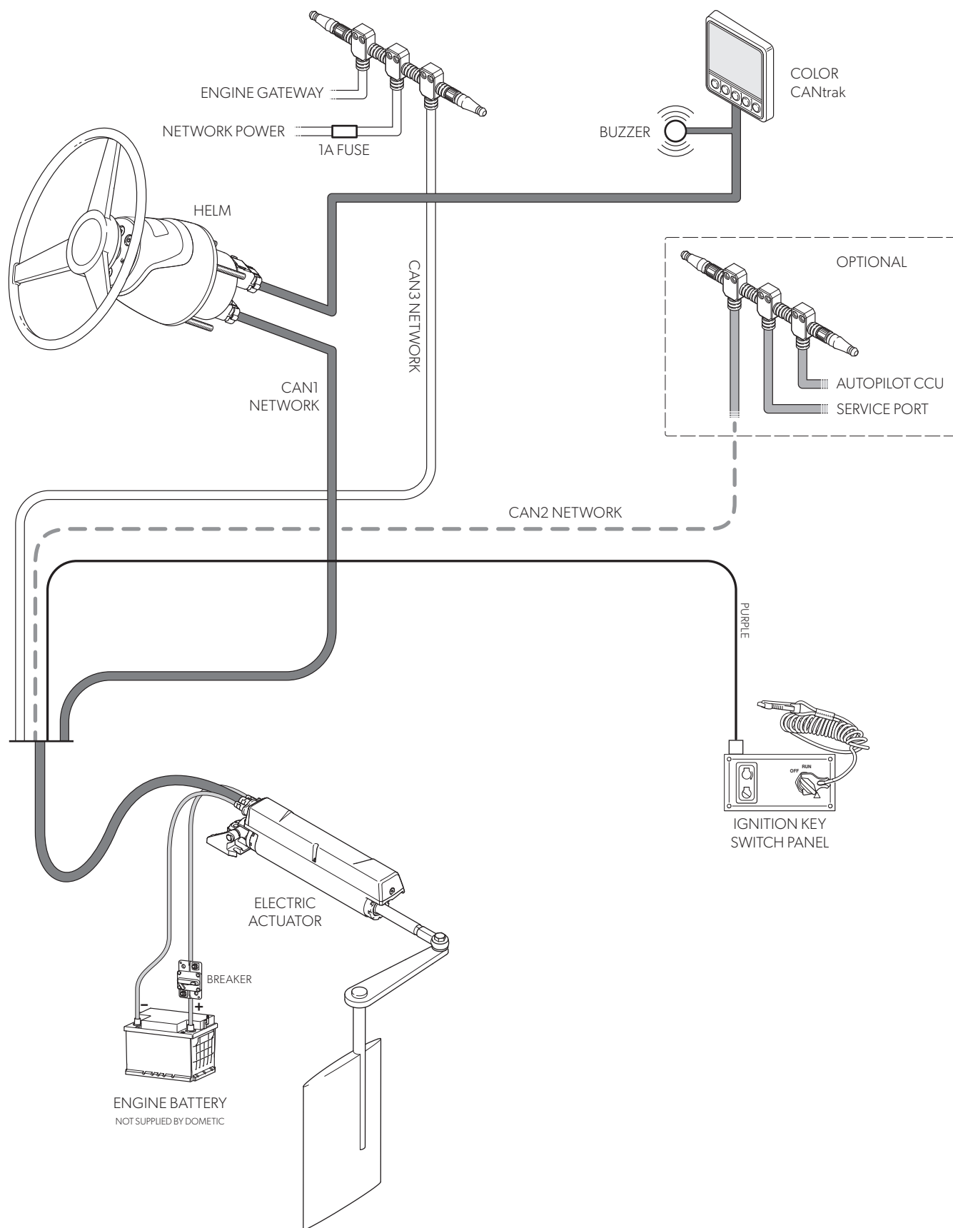
Figure 10-12. Electric inboard system diagram, single actuator (for reference only).
