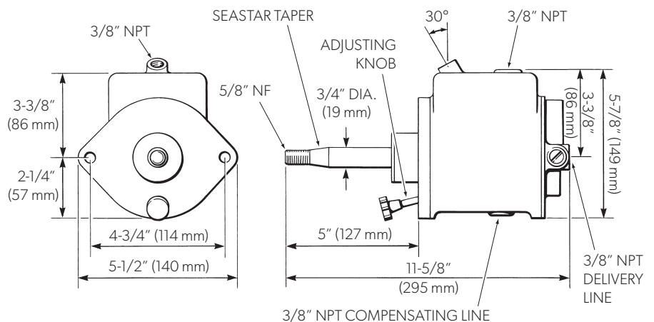
Figure 7-13. Uses remote fill kit HA5450.
