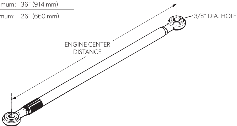
Figure 3-32. Tie bar part # HO5009.
