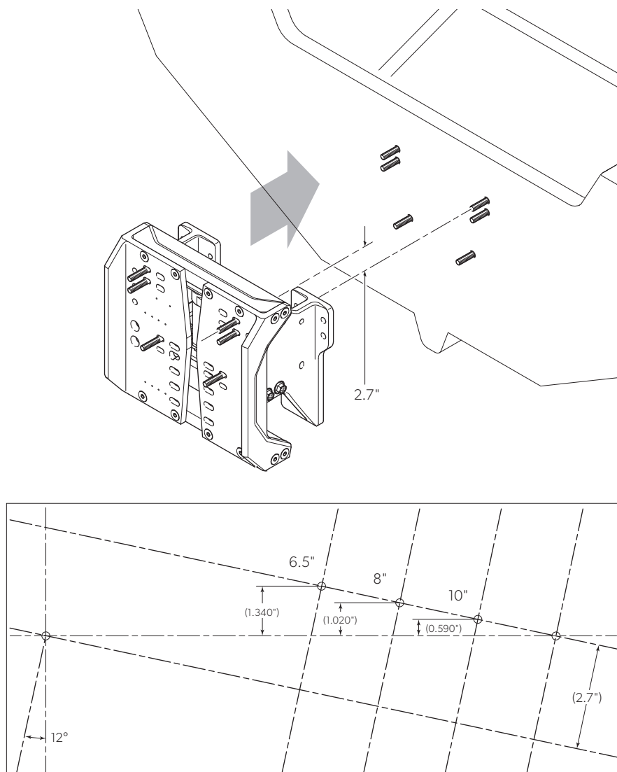
Figure 13-7. Engine lift per setback — Standard (OMC) Mega jack plate. Not to scale.
