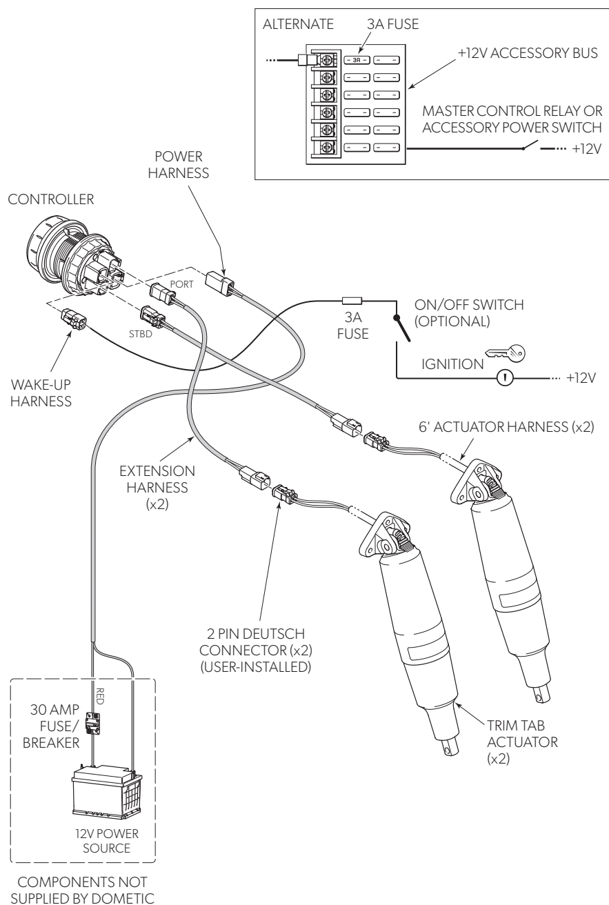
Figure 12-7. Single station (standard series shown).
