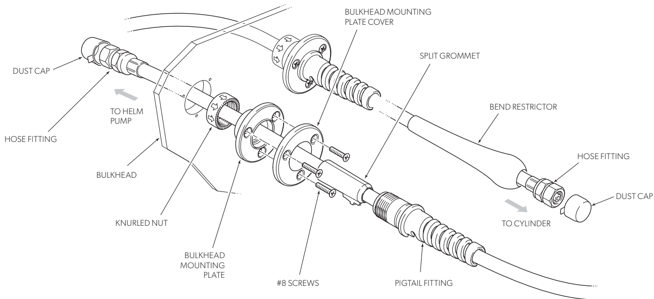
Figure 9-2. Field installed bulkhead, single hose kit, stainless bezels shown.
