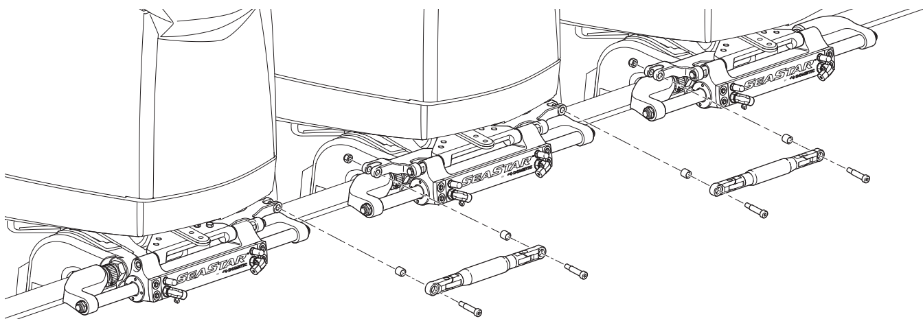
Figure 3-27. Triple engine – triple cylinder configuration.
