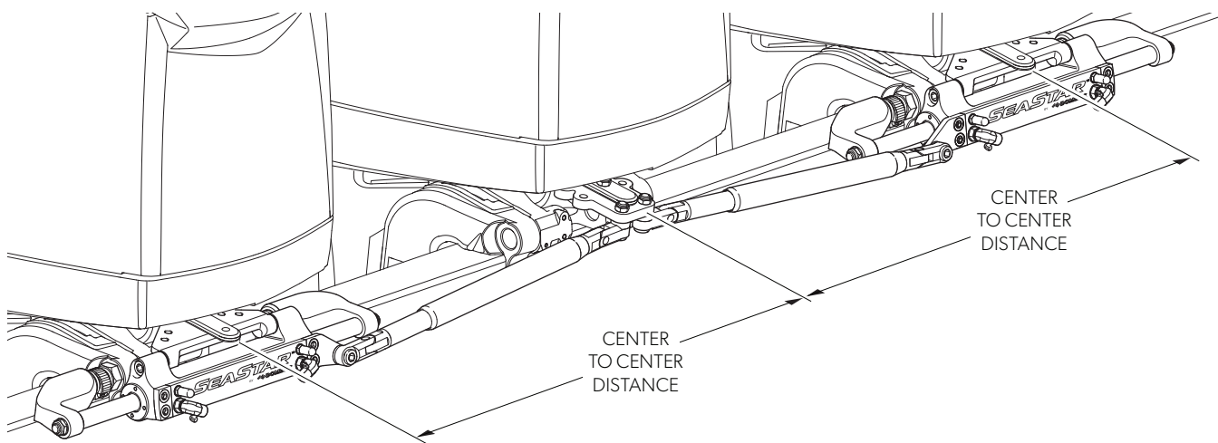
Figure 3-26. Triple engine – dual cylinder configuration.
