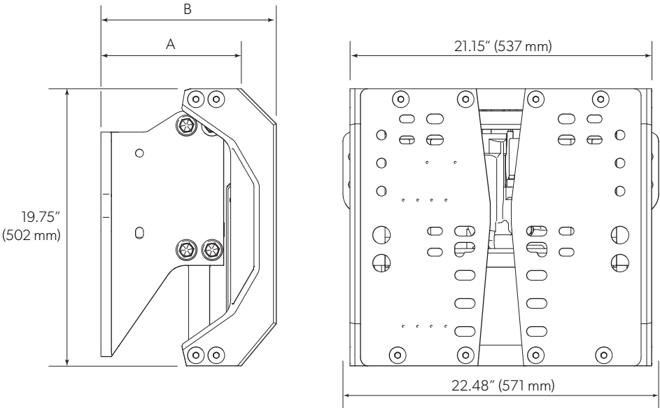
Figure 13-5. Standard (OMC) Mega jack plate.
