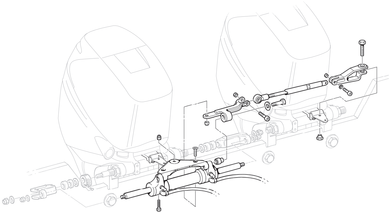
Figure 3-14. Tie bar kit # HO6001 shown, is used for most single cylinder twin engine applications. See 3.2.6.
