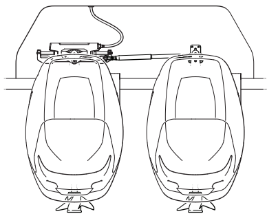
Figure 10-1. Single actuator twin engines.
