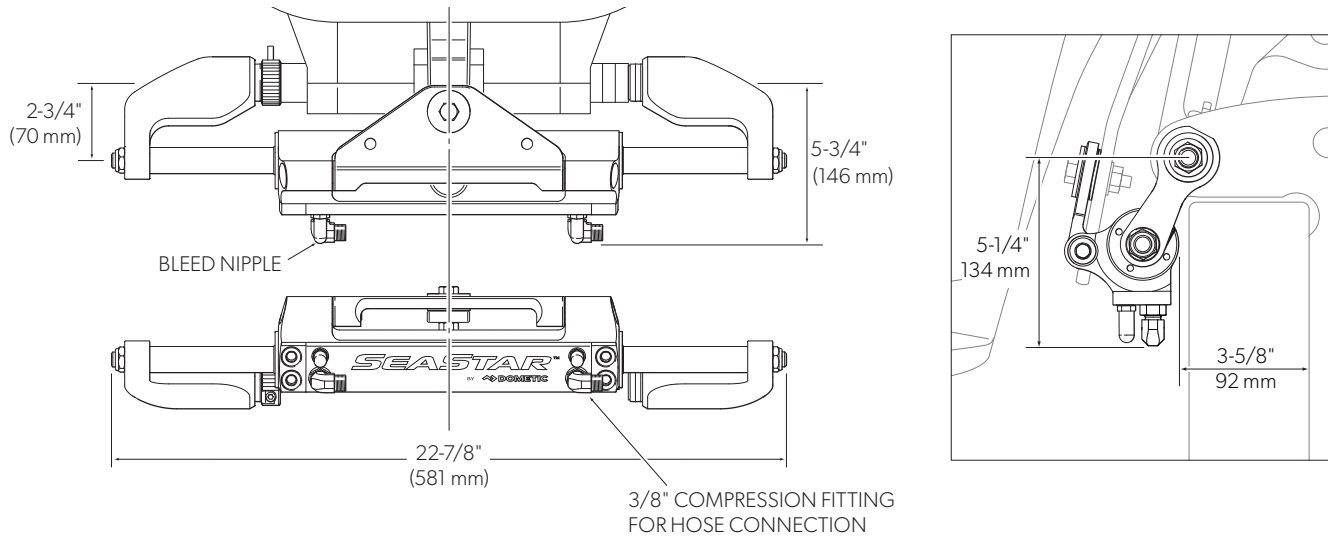
Figure 3-28. Tournament cylinder dimensions.
