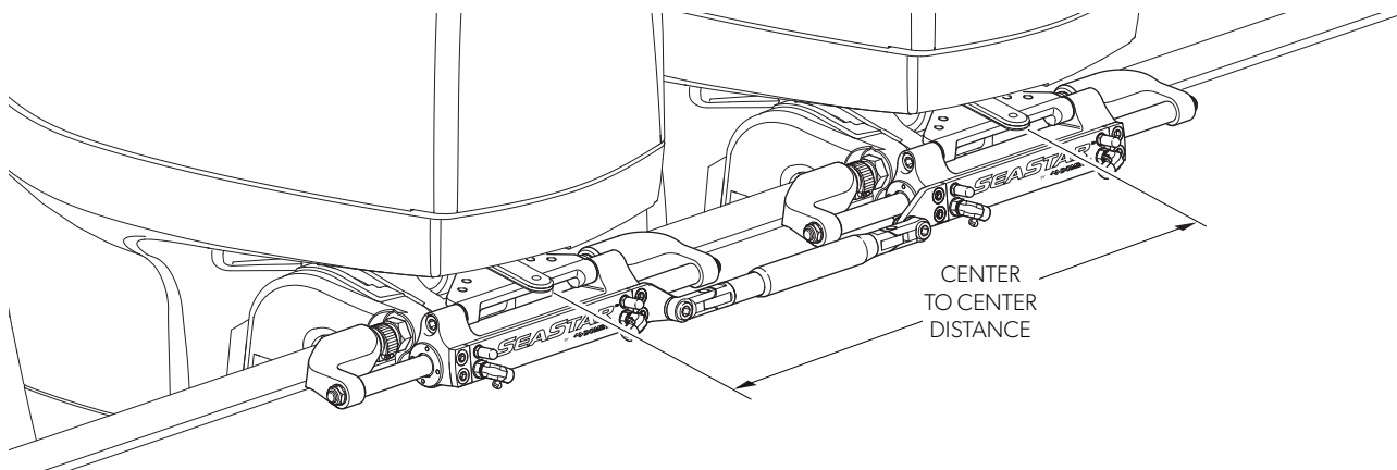
Figure 3-25. Twin engine – dual cylinder configuration
