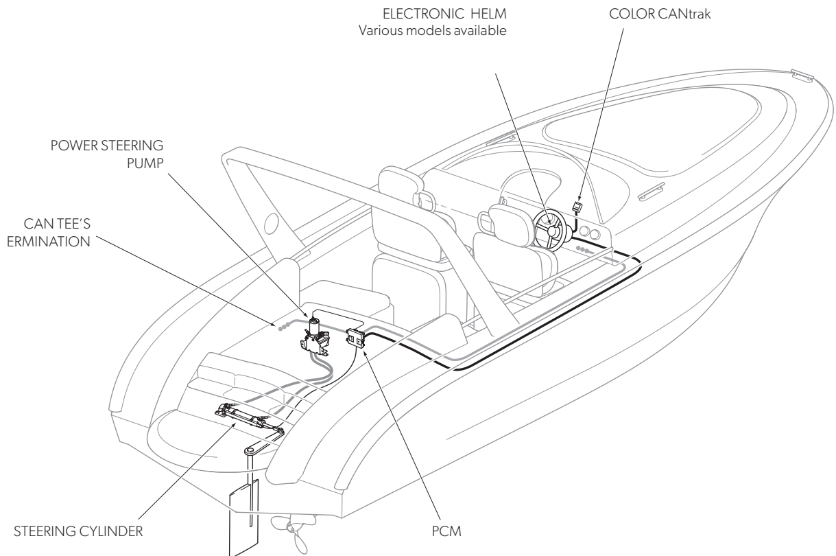
Figure 11-1. System components. Single rudder system shown. * Subject to submission of survey form and rudder load calculation.
