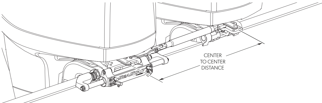
Figure 3-24. Twin engine – single cylinder (starboard) configuration.
