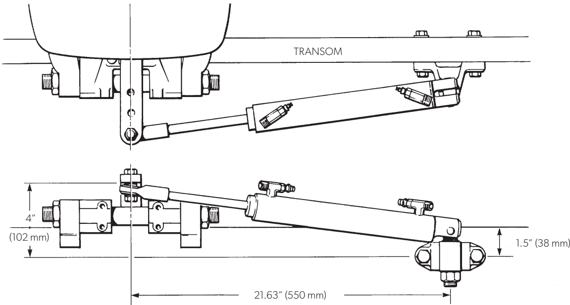
Figure 3-35. Splashwell mount cylinder part # HC5380-3.
