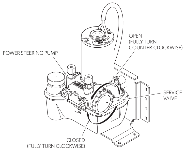
Figure 10-22. Service valve location.
