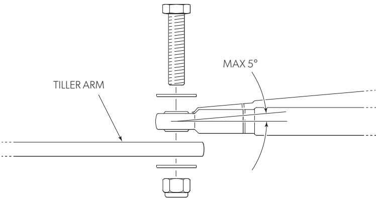
Figure 10-11. Electric inboard actuator attachment to tiller arm, recommended per ABYC.
