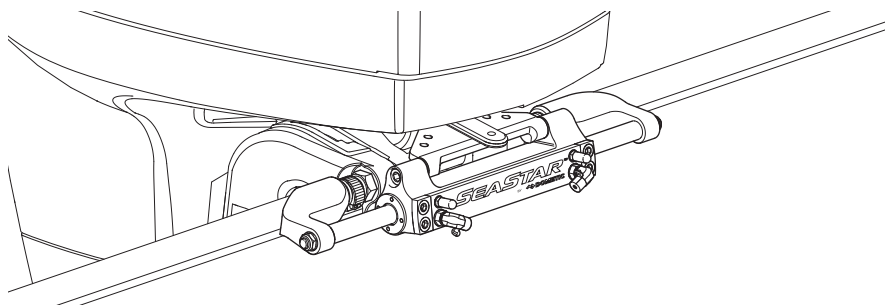
Figure 3-23. Single engine – single cylinder configuration.
