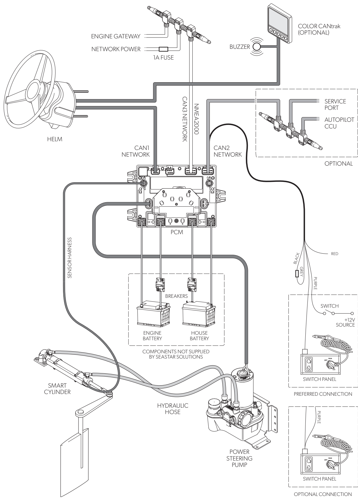
Figure 11-3. Optimus EPS system diagram, single station, single rudder.
