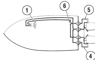
Figure I. Dual side mount cylinders
