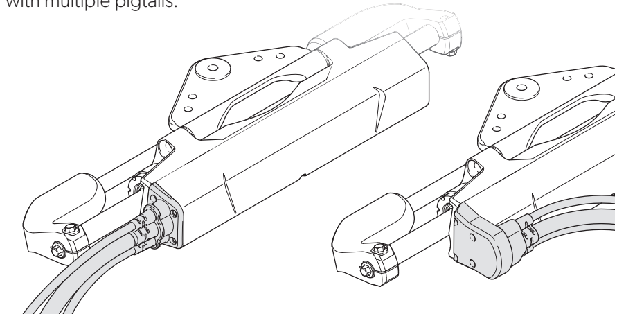
Figure 10-4. Straight actuator harness, and 180° actuator harness.
