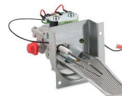
Natural Gas Conversion Kit 40K Models Only Item #9630002231 Side Mount Extended Manifold - All Models Item #9630002330
