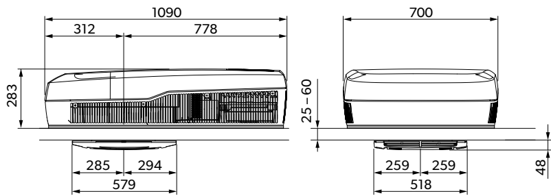
FreshJet FJX7457IHP
