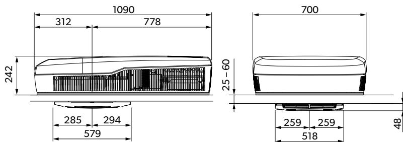
FreshJet FJX7337IHP
