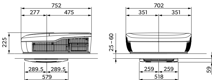
FreshJet FJX4233M
