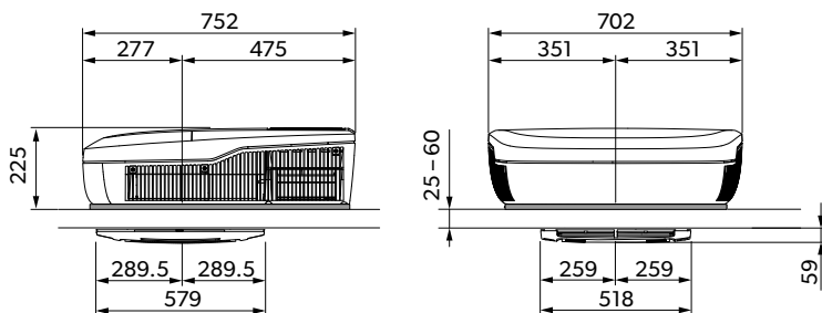
FreshJet FJX4233M
