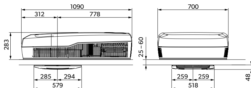
FreshJet FJX7457IHP
