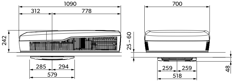
FreshJet FJX7337IHP
